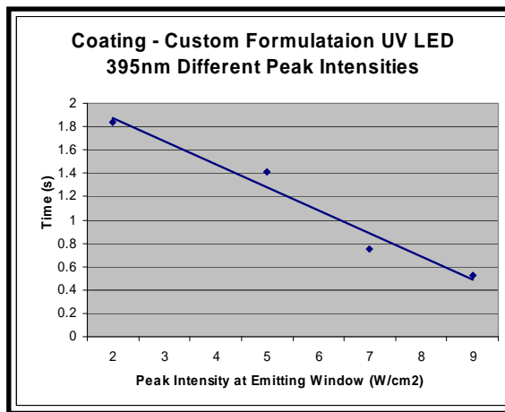
Figure 19: Linear relationship 395nm, 365nm and Peak Intensity vs. Cure Rate
