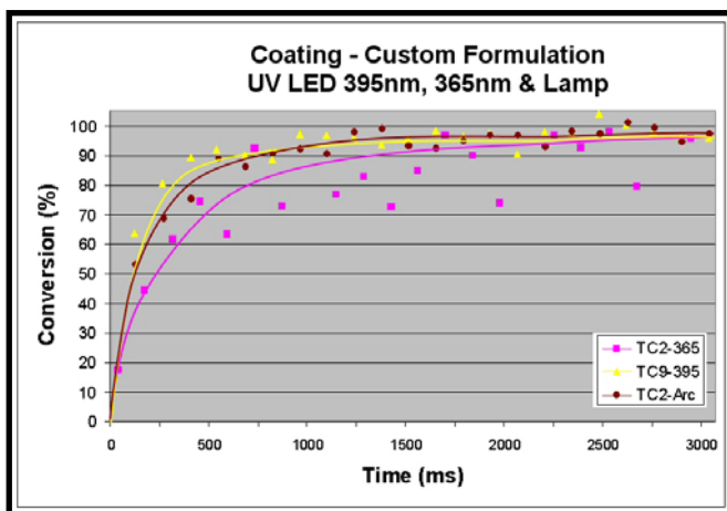
Figure 17: Conversion Rate for UV LED 395nm, 365nm and Mercury vapor Lamp
