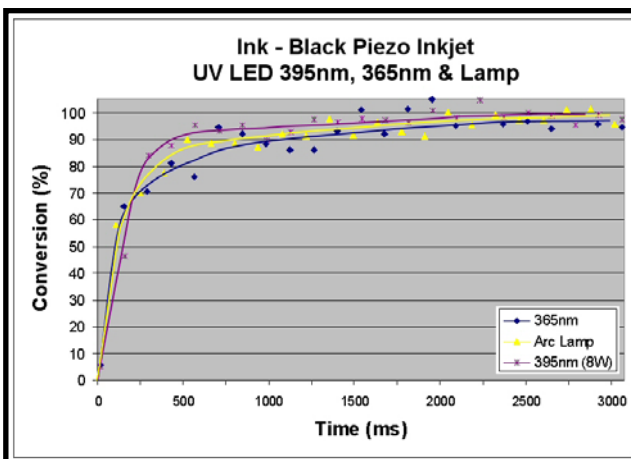
Figure 11: Conversion Rate for UV LED 395nm, 365nm and Mercury Vapor Lamp
