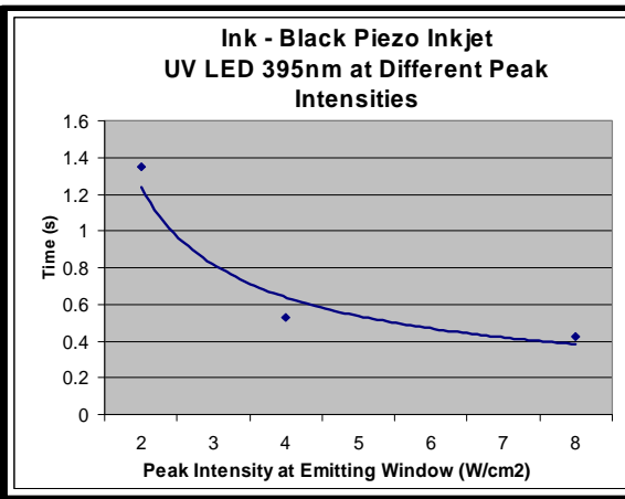
Figure 10: Non-linear Relationship Peak Intensity vs. Cure Rate
