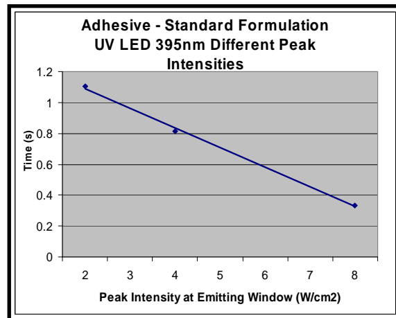
Figure 14: Linear relationship between Peak Intensity and Cure Rate
