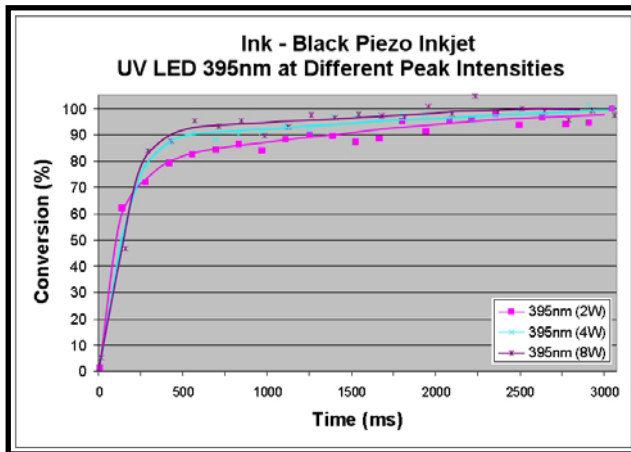
Figure 9: UV LED 395nm UV Source at Different Peak Intensities curing black ink
