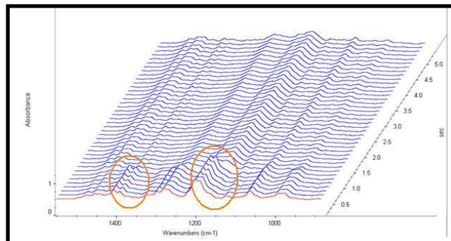
Figure 6: Absorbance versus Wavenumber FTIR Plot for Ink Sample
