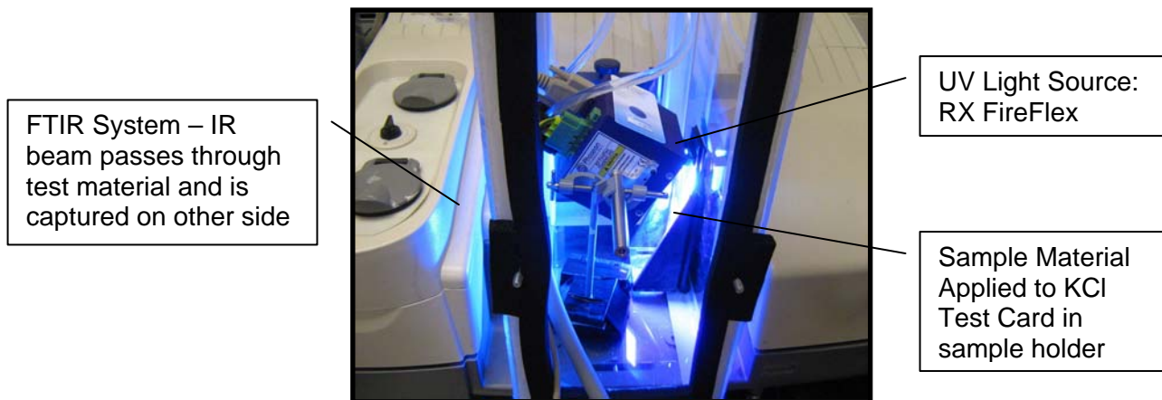
Figure 5: FTIR System Setup
