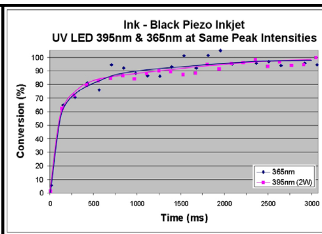
Figure 12: Conversion Rate for UV LED Sources 395nm and 365nm at Same Intensity
