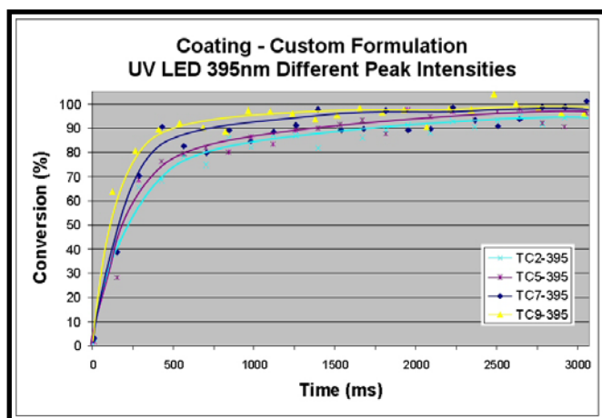
Figure 18: Conversion Rate for UV LED Mercury Vapor Lamp
