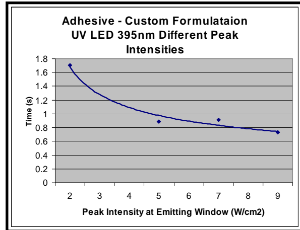
Figure 16: Non-linear relationship between Peak Intensity and Cure Rate
