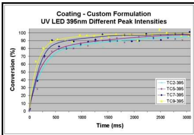
Figure 12: Conversion Rate for UV LED
