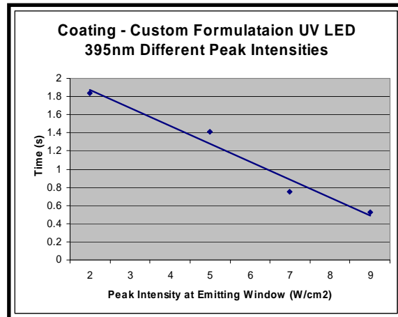
Figure 13: Linear relationship 395nm, 365nm and Mercury Vapour Lamp Peak Intensity vs. Cure Rate
