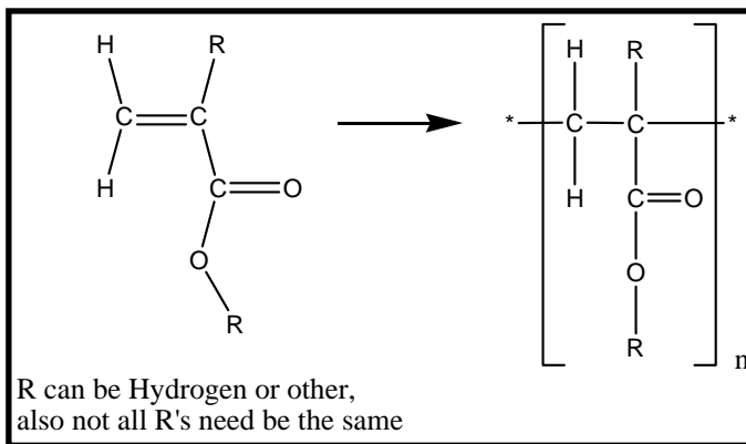
Figure 10: Depiction of C=C bond reaction in acrylate group
